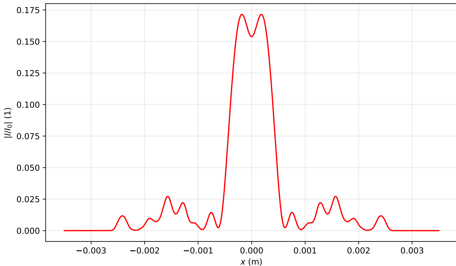
Intensity profile I(x, y = 0, z = 3.105)/I_0 , P_{in}=11.0\text{Pcr} , artificial time
