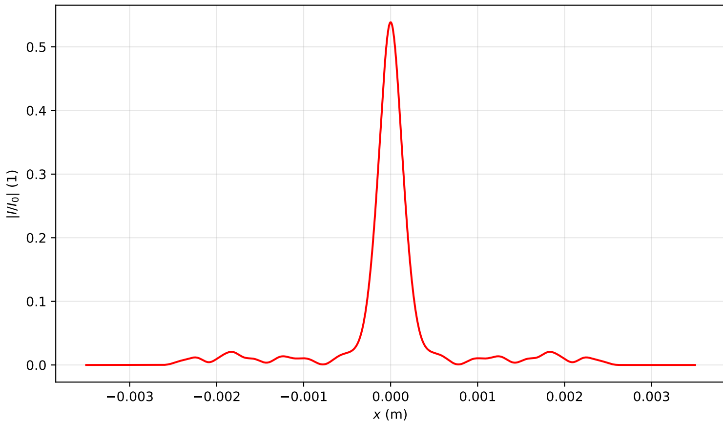
Intensity profile I(x, y = 0, z = 3.582)/I_0 , P_{in}=11.0P_{cr} , artificial time
