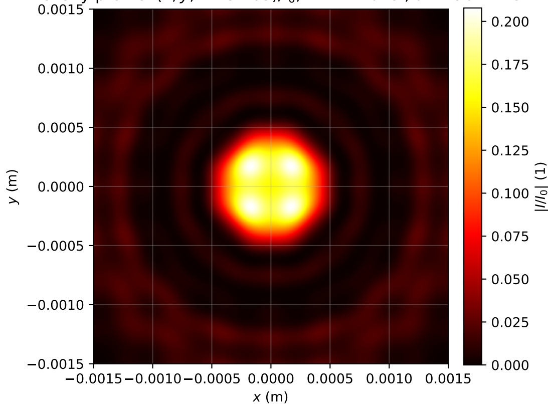
Intensity profile I(x, y, z = 3.105)/I_0 , P_{in}=11.0P_{cr} , artificial time
