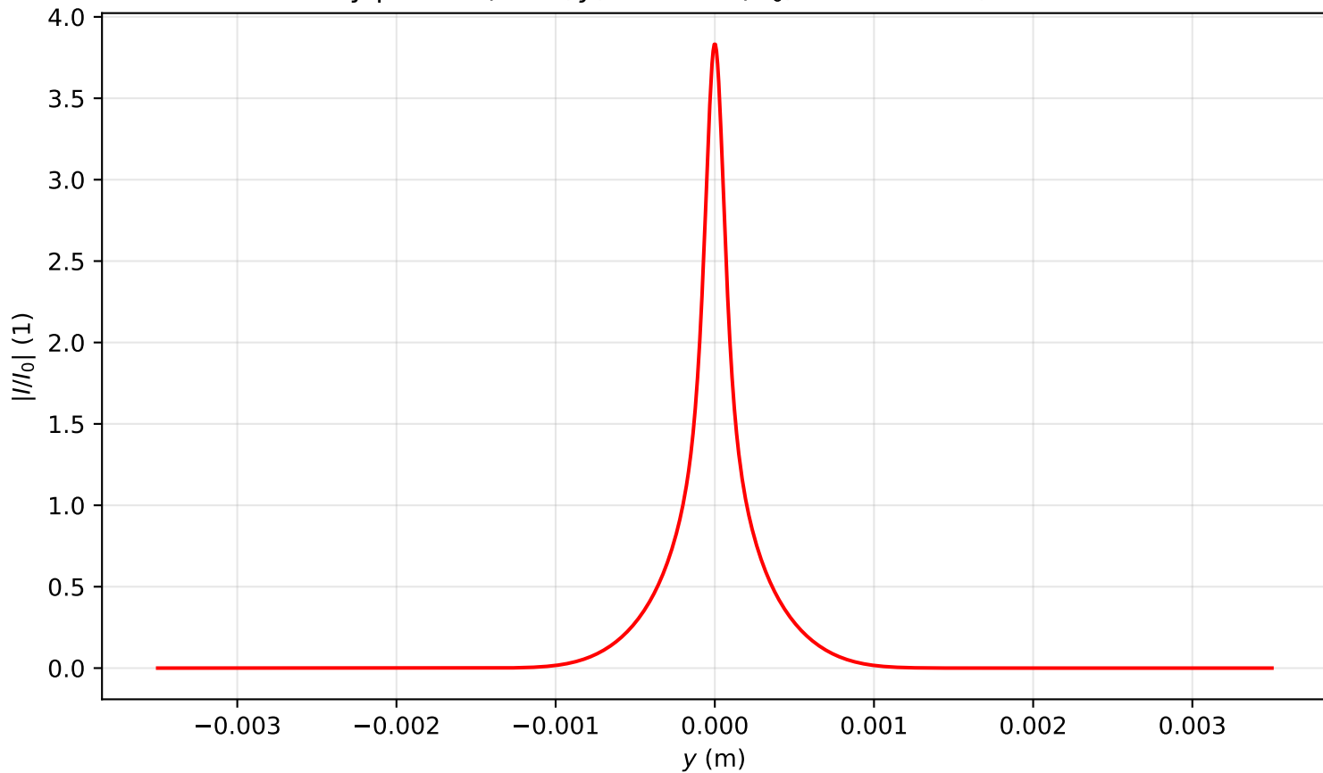
Intensity profile I(x=0, y, z=0.239)/I_0 , P_{in}=11.0P_{cr} , artificial time
