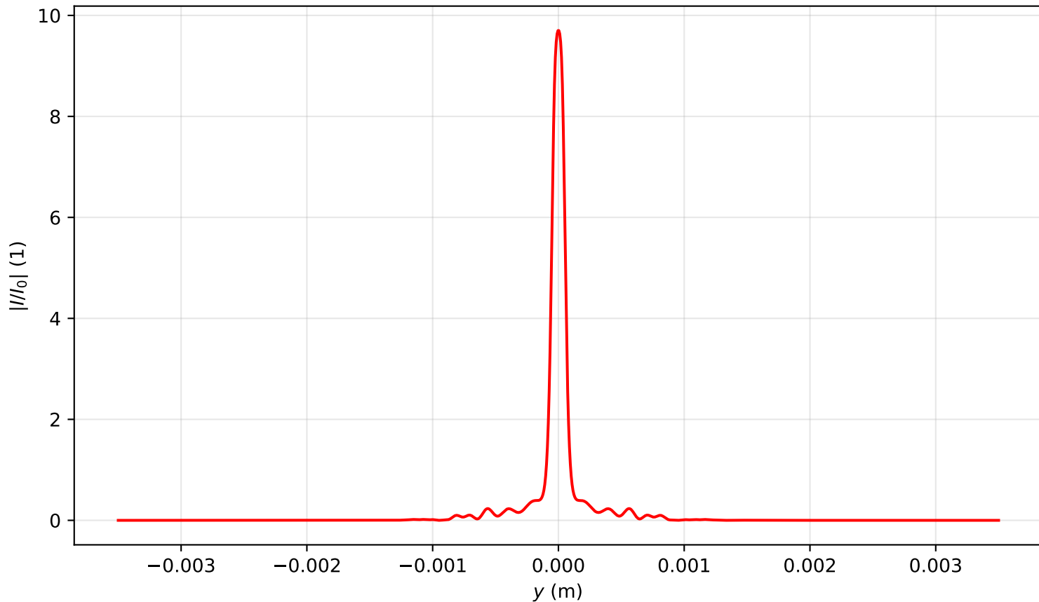
Intensity profile I(x=0, y, z=0.716)/I_0 , P_{in}=11.0P_{cr} , artificial time
