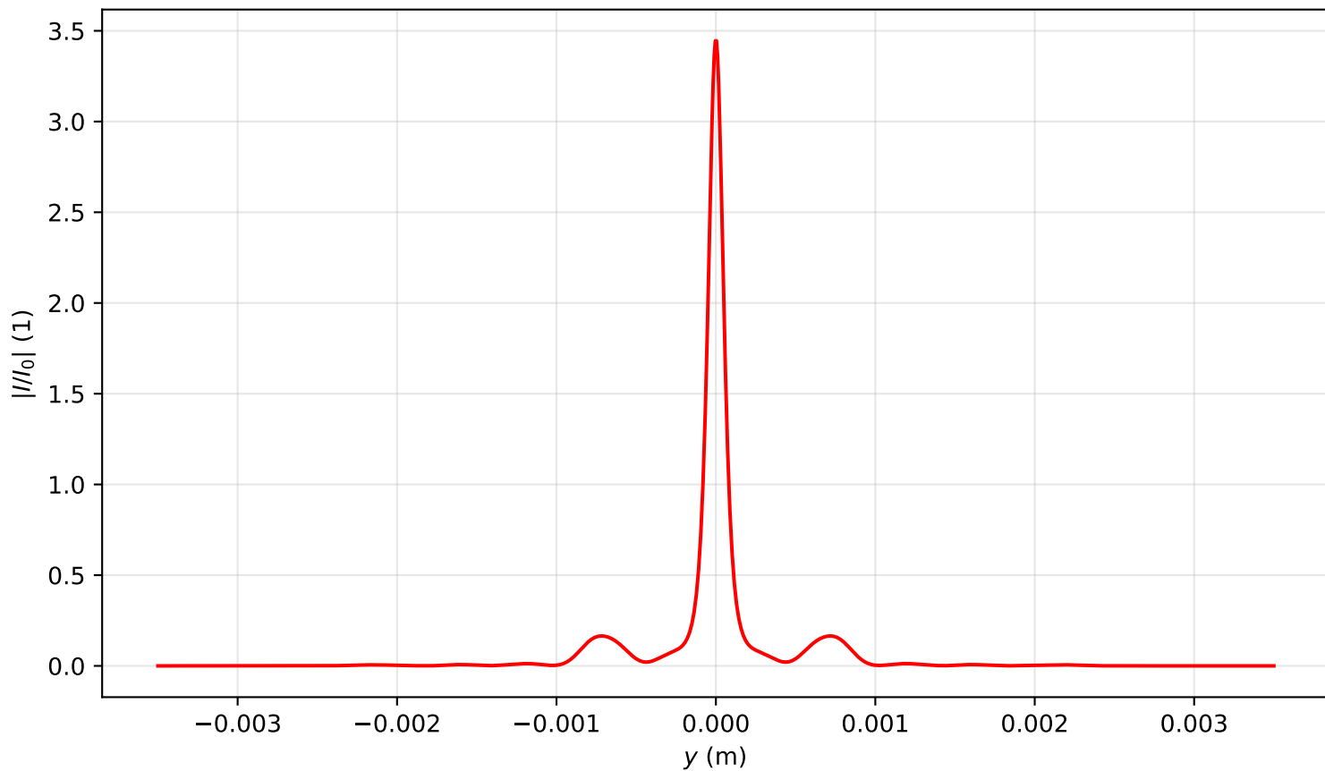
Intensity profile I(x=0, y, z=1.194)/I_0 , P_{in}=11.0P_{cr} , artificial time
