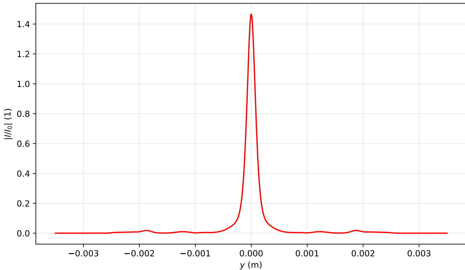
Intensity profile I(x=0, y, z=3.821)/I_0 , P_{in}=11.0P_{cr} , artificial time
