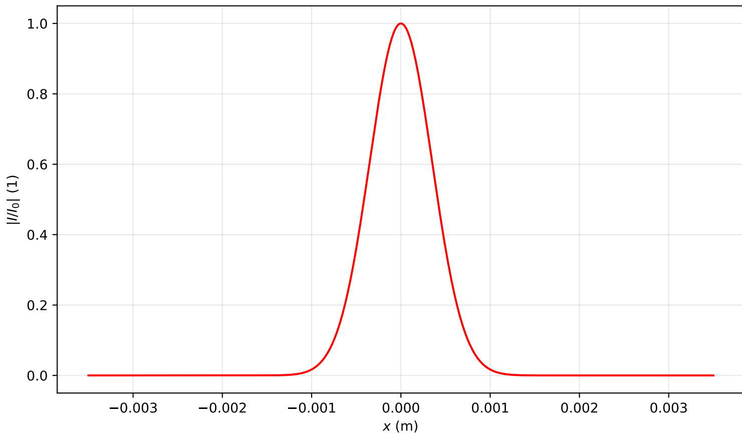
Intensity profile I(x, y = 0, z = 0.000)/I_0 , P_{in}=11.5P_{cr} , artificial time
