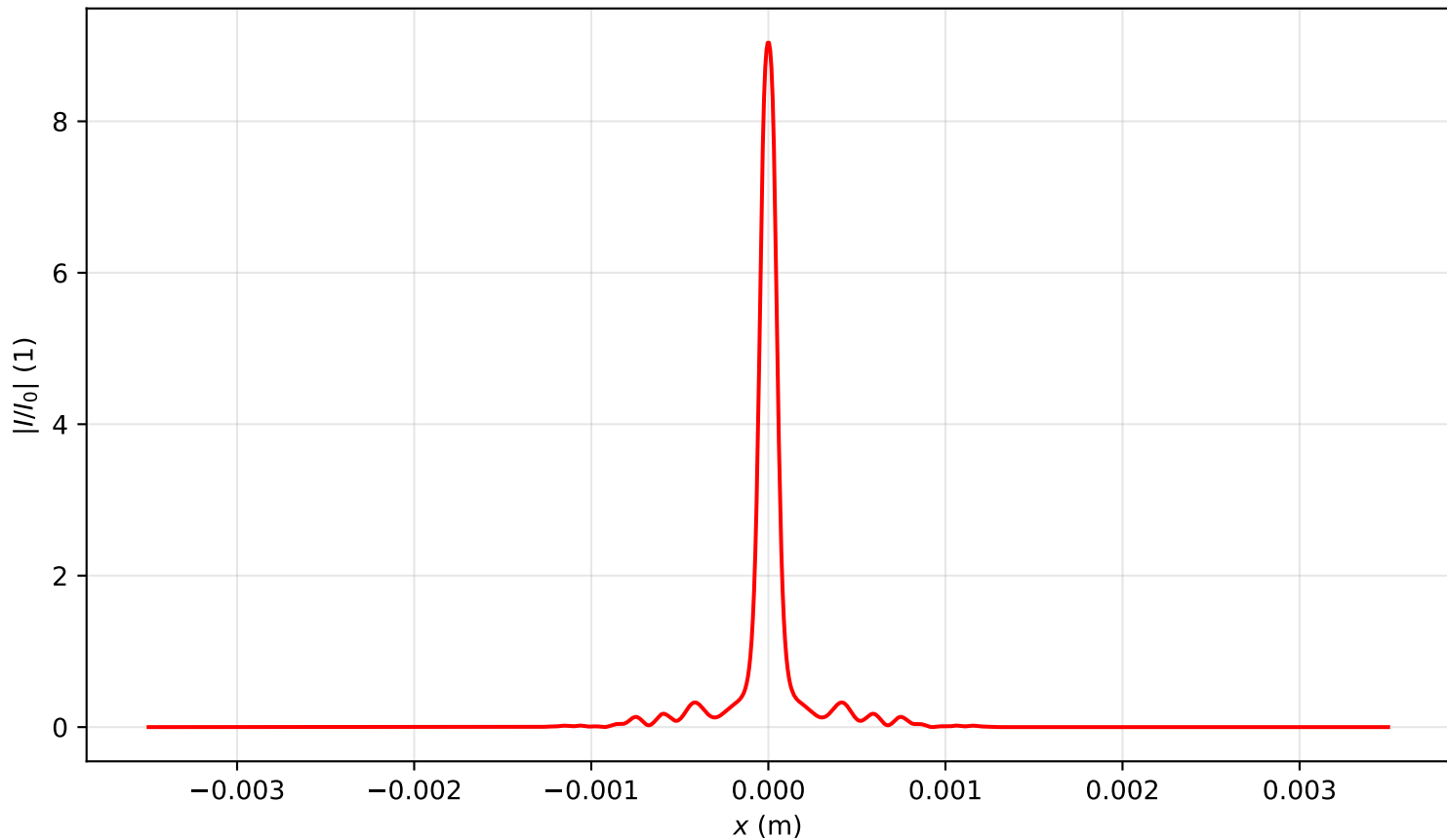
Intensity profile I(x, y = 0, z = 0.716)/I_0 , P_{in}=11.5P_{cr} , artificial time
