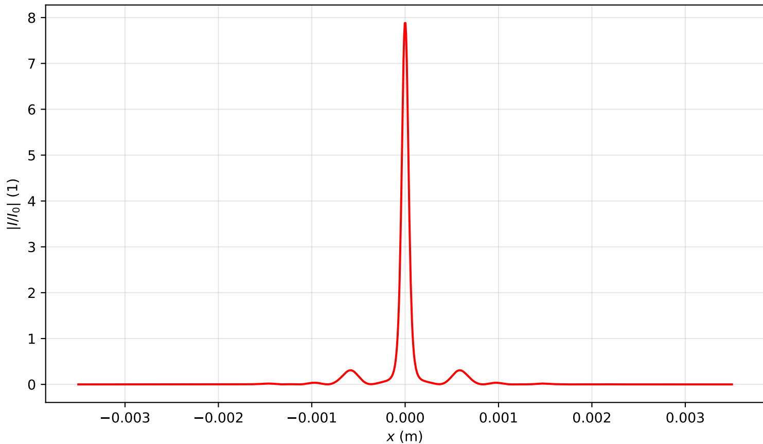
Intensity profile I(x, y = 0, z = 0.955)/I_0 , P_{in}=11.5P_{cr} , artificial time
