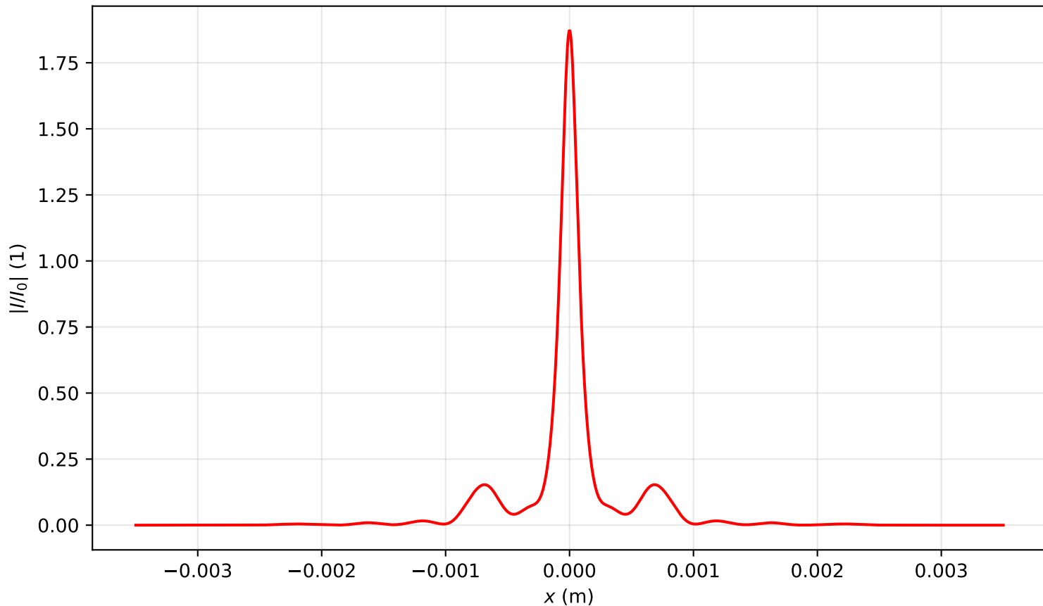
Intensity profile I(x, y = 0, z = 1.194)/I_0 , P_{in}=11.5P_{cr} , artificial time
