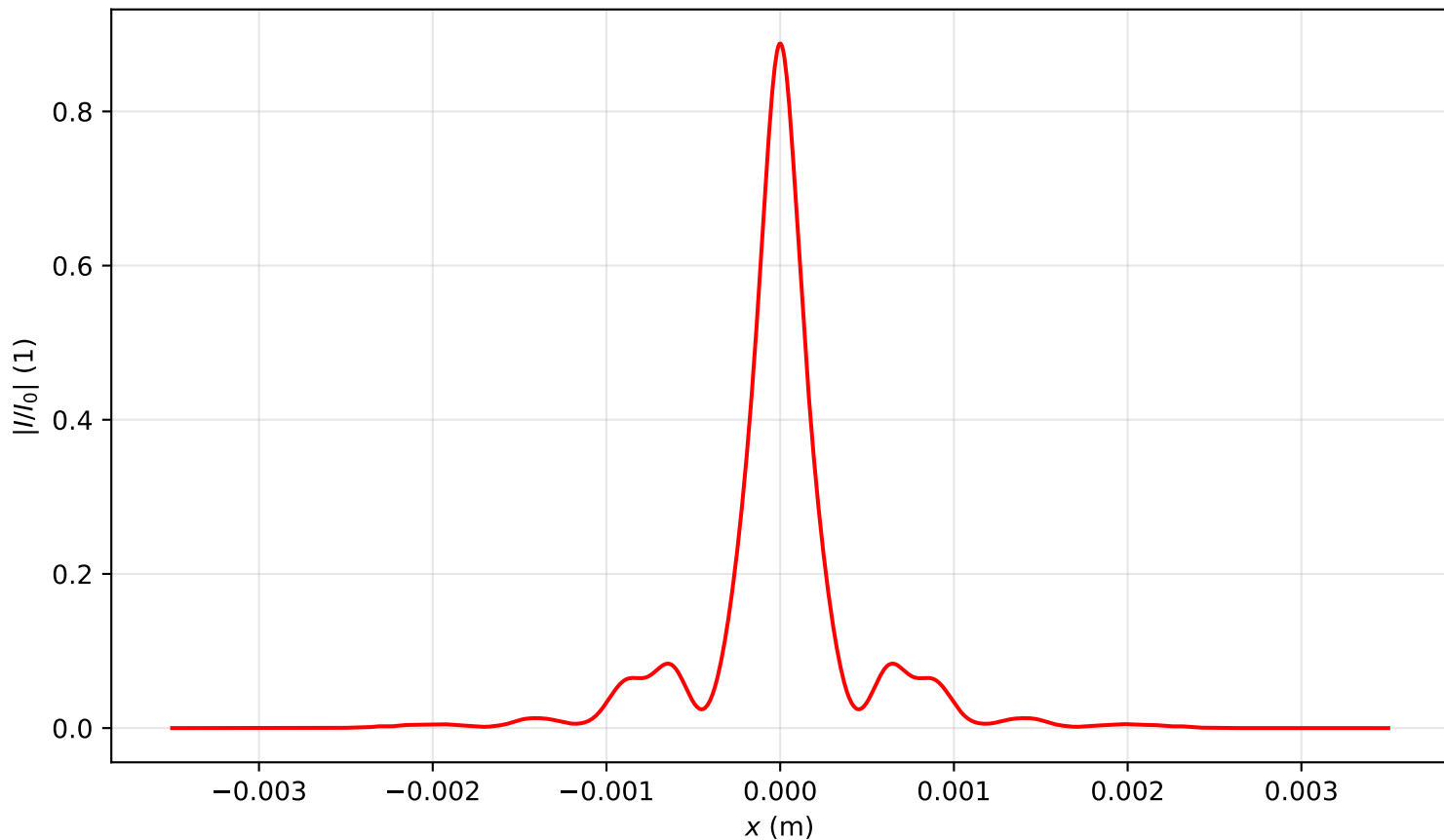
Intensity profile I(x, y = 0, z = 1.433)/I_0 , P_{in}=11.5P_{cr} , artificial time
