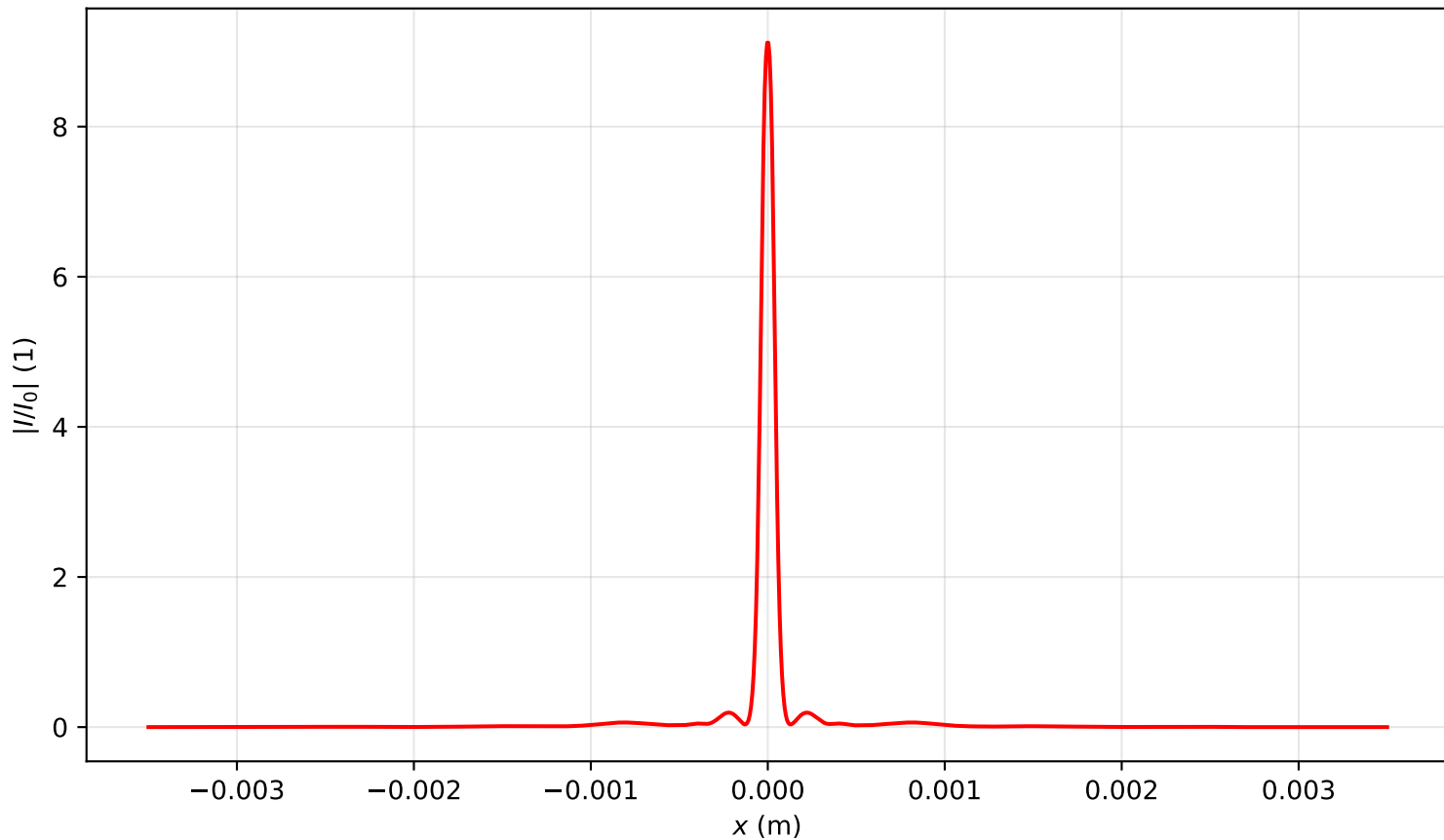
Intensity profile I(x, y = 0, z = 1.672)/I_0 , P_{in}=11.5P_{cr} , artificial time
