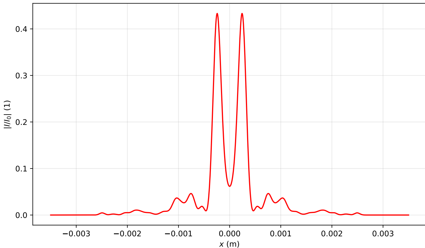
Intensity profile I(x, y = 0, z = 1.911)/I_0 , P_{in}=11.5P_{cr} , artificial time
