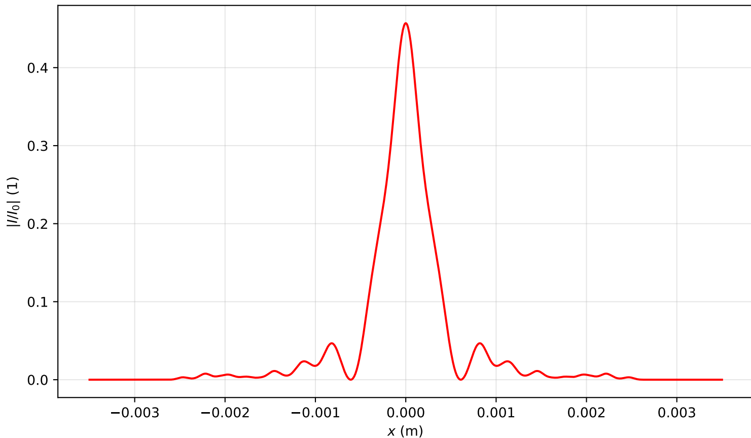
Intensity profile I(x, y = 0, z = 2.149)/I_0 , P_{in}=11.5P_{cr} , artificial time
