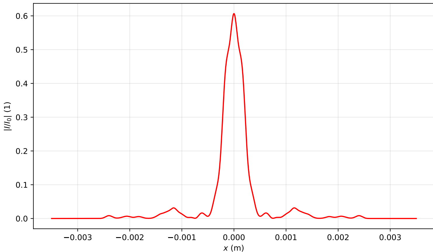
Intensity profile I(x, y = 0, z = 2.627)/I_0 , P_{in}=11.5P_{cr} , artificial time
