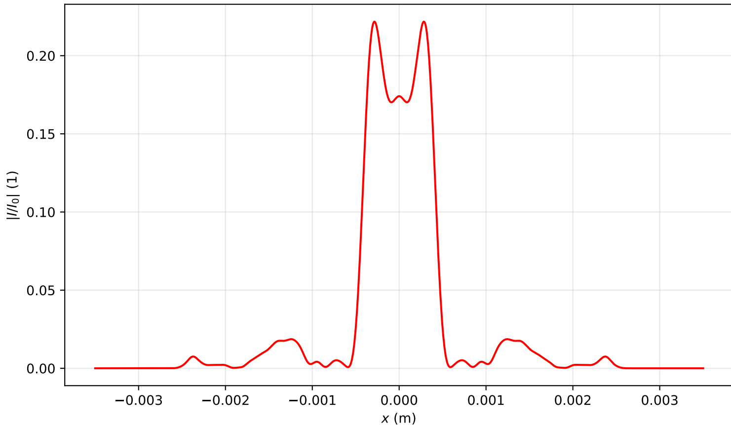
Intensity profile I(x, y = 0, z = 2.866)/I_0 , P_{in}=11.5P_{cr} , artificial time
