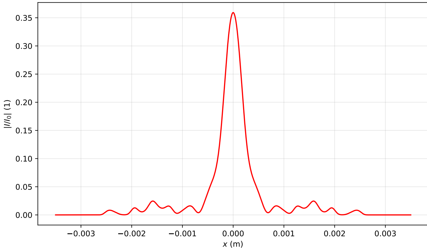
Intensity profile I(x, y = 0, z = 3.105)/I_0 , P_{in}=11.5P_{cr} , artificial time
