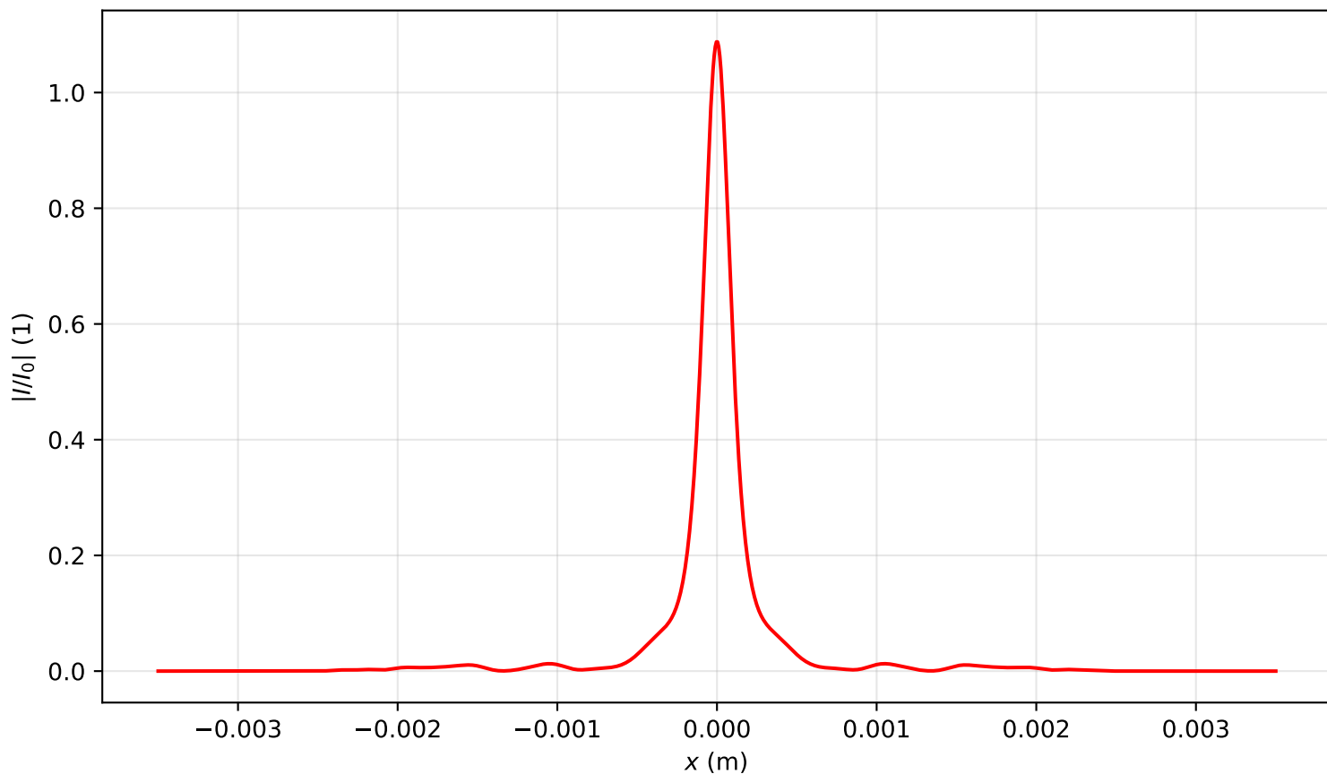
Intensity profile I(x, y = 0, z = 3.344)/I_0 , P_{in}=11.5P_{cr} , artificial time
