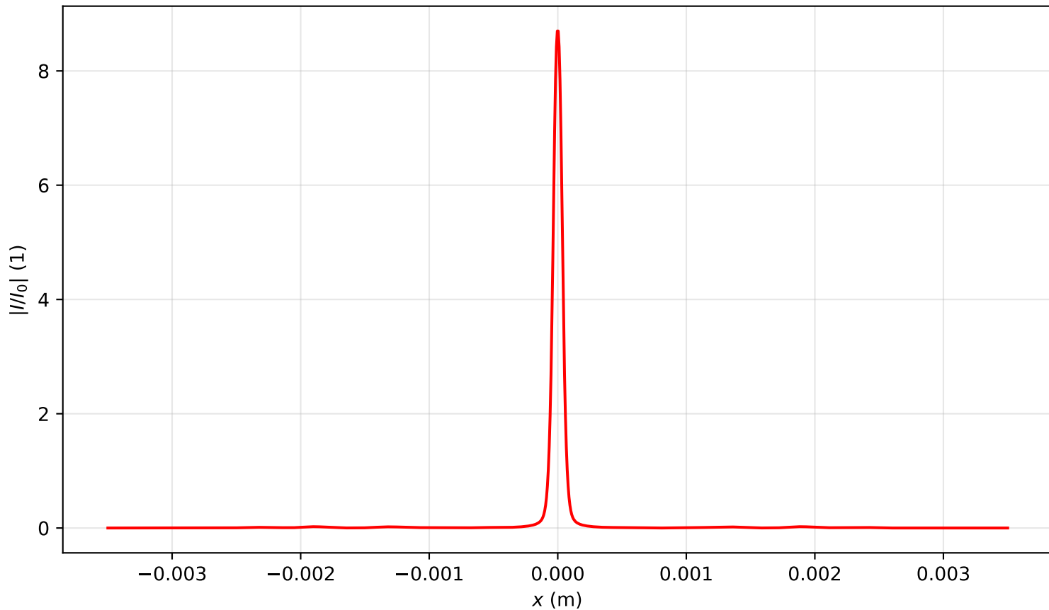
Intensity profile I(x, y = 0, z = 3.582)/I_0 , P_{in}=11.5P_{cr} , artificial time
