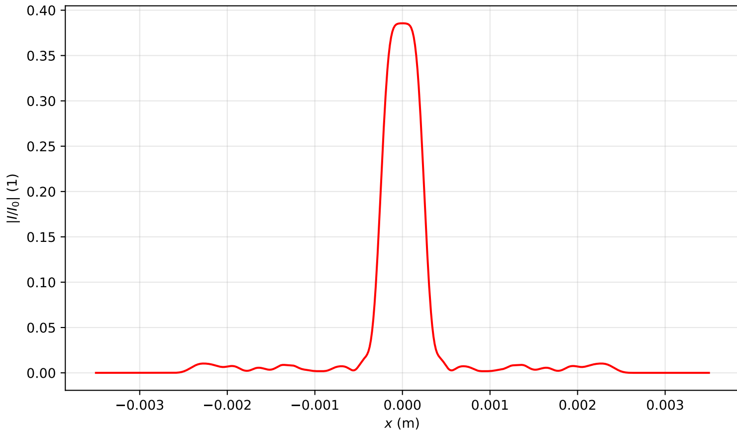
Intensity profile I(x, y = 0, z = 3.821)/I_0 , P_{in}=11.5P_{cr} , artificial time
