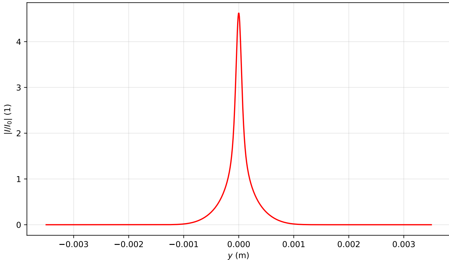
Intensity profile I(x=0, y, z=0.239)/I_0 , P_{in}=11.5P_{cr} , artificial time
