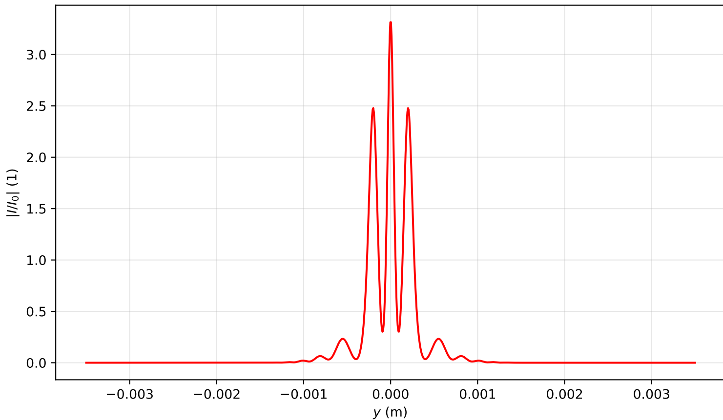
Intensity profile I(x=0, y, z=0.478)/I_0 , P_{in}=11.5P_{cr} , artificial time
