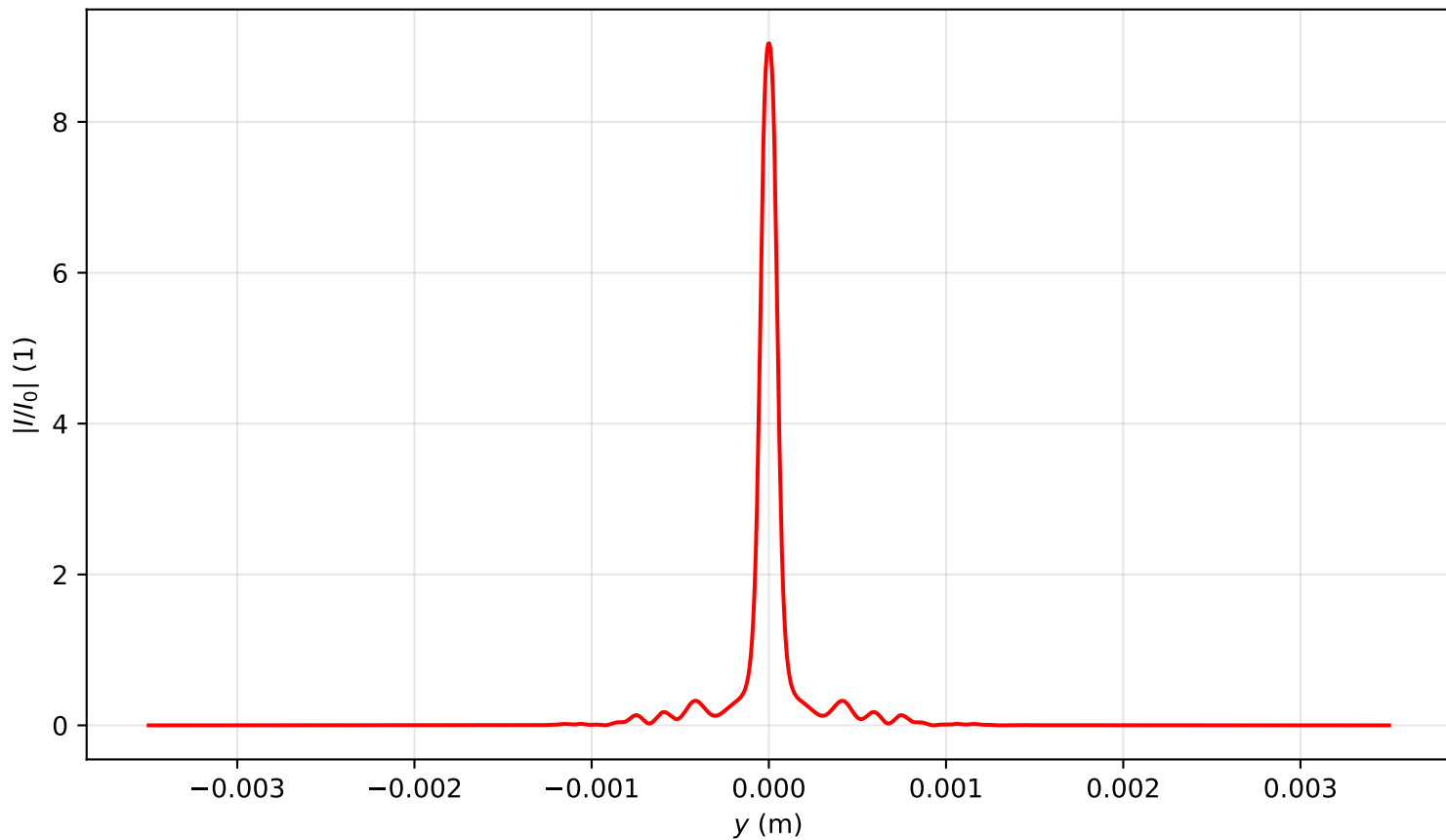
Intensity profile I(x=0, y, z=0.716)/I_0 , P_{in}=11.5P_{cr} , artificial time
