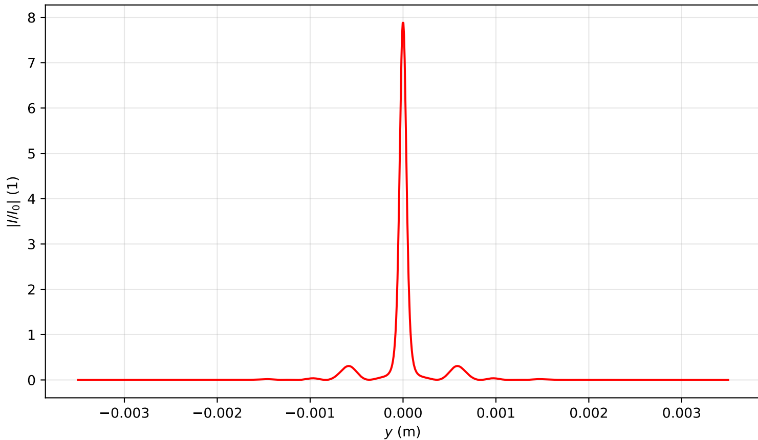
Intensity profile I(x=0, y, z=0.955)/I_0 , P_{in}=11.5P_{cr} , artificial time
