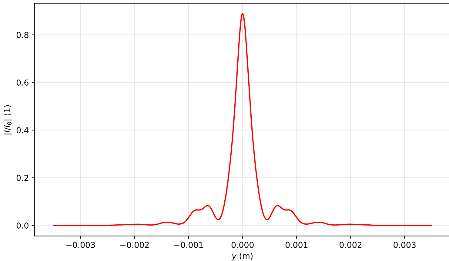
Intensity profile I(x=0, y, z=1.433)/I_0 , P_{in}=11.5P_{cr} , artificial time
