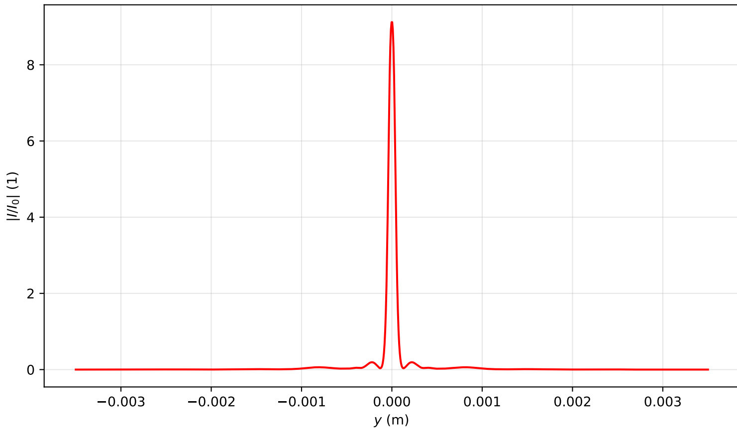
Intensity profile I(x=0, y, z=1.672)/I_0 , P_{in}=11.5P_{cr} , artificial time
