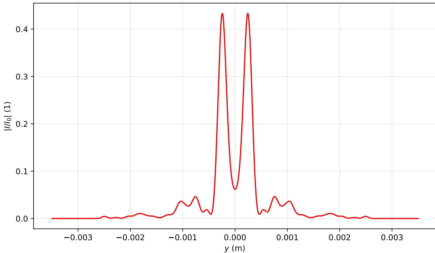
Intensity profile I(x=0, y, z=1.911)/I_0 , P_{in}=11.5P_{cr} , artificial time
