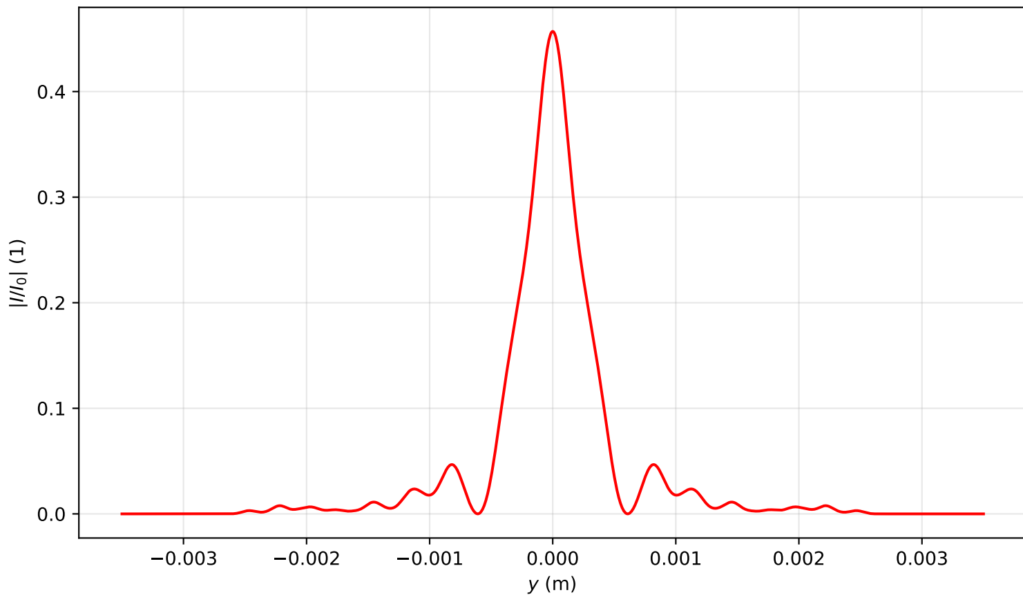
Intensity profile I(x=0, y, z=2.149)/I_0 , P_{in}=11.5P_{cr} , artificial time
