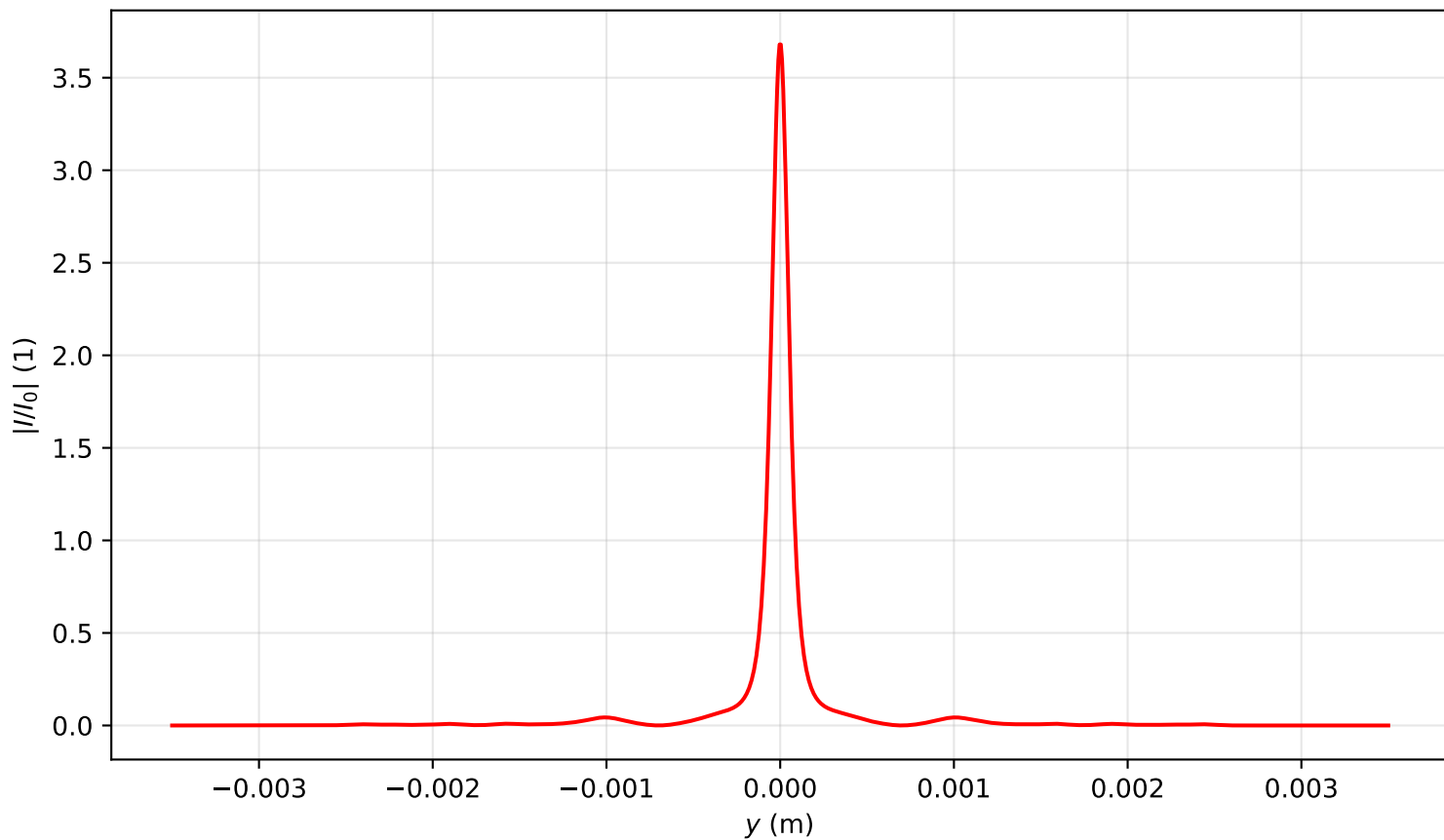
Intensity profile I(x=0, y, z=2.388)/I_0 , P_{in}=11.5P_{cr} , artificial time
