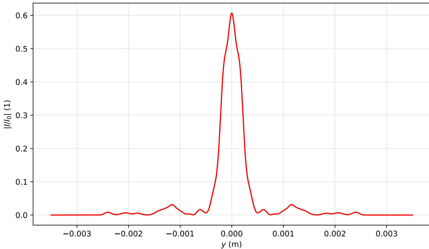
Intensity profile I(x=0, y, z=2.627)/I_0 , P_{in}=11.5P_{cr} , artificial time
