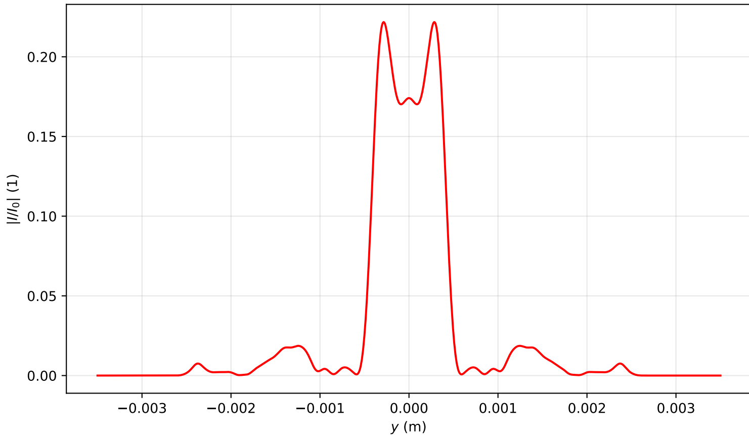
Intensity profile I(x=0, y, z=2.866)/I_0 , P_{in}=11.5P_{cr} , artificial time
