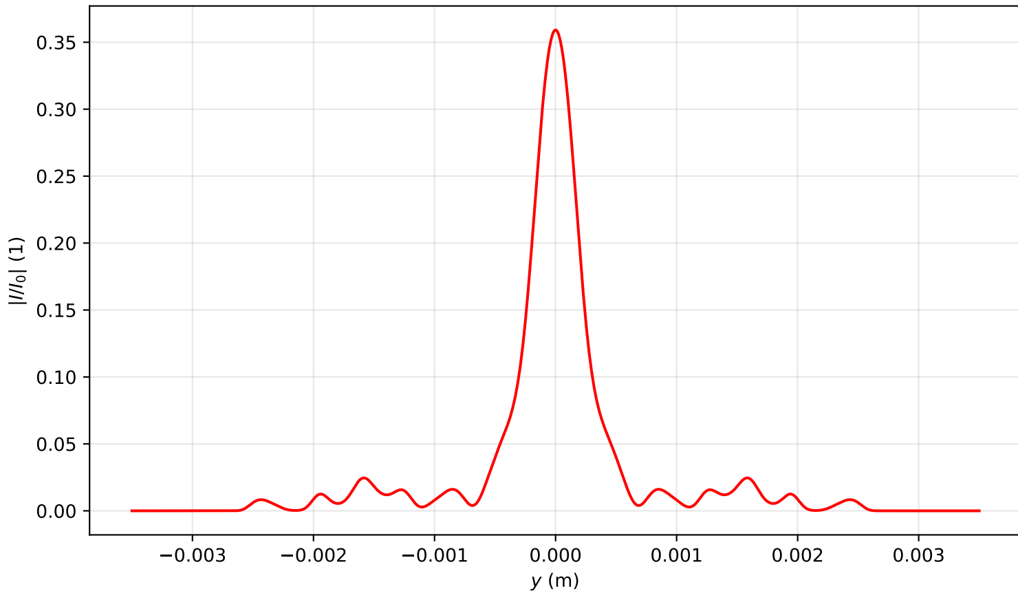
Intensity profile I(x=0, y, z=3.105)/I_0 , P_{in}=11.5P_{cr} , artificial time
