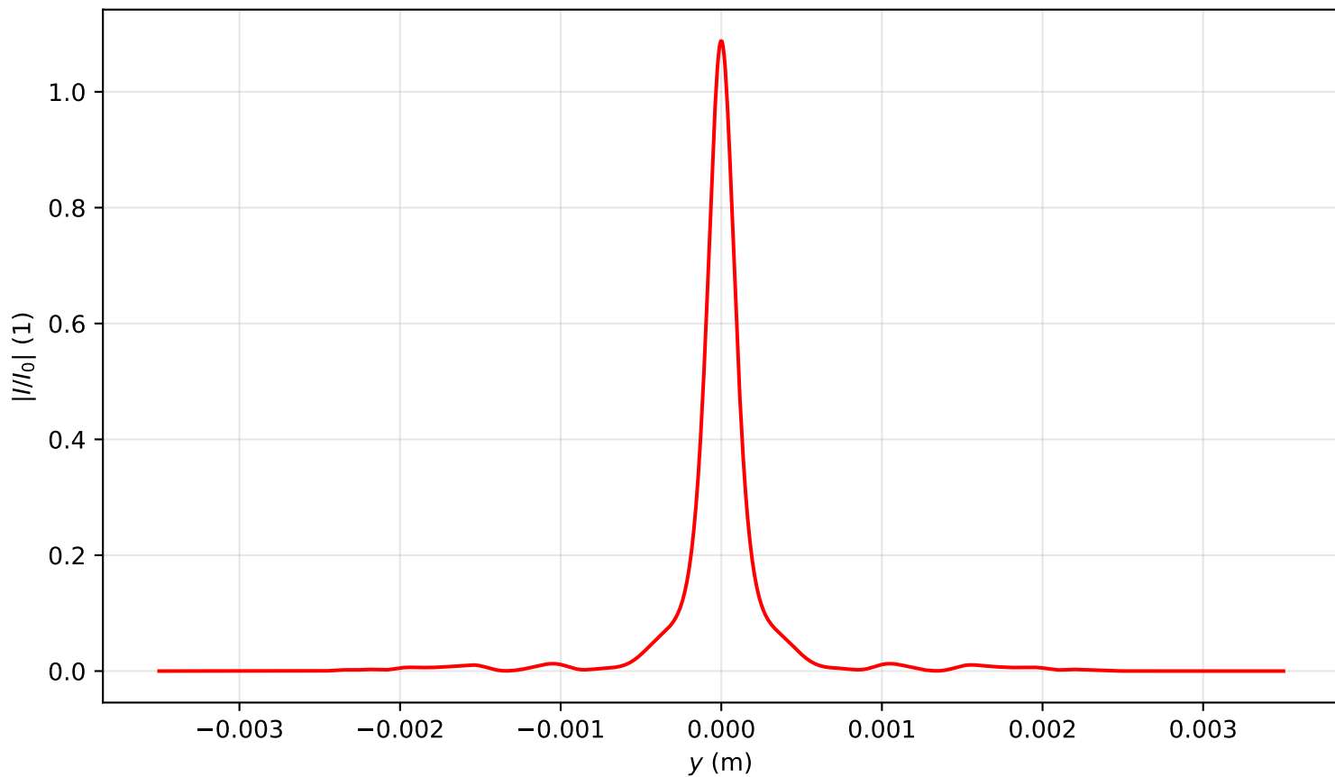
Intensity profile I(x=0, y, z=3.344)/I_0 , P_{in}=11.5P_{cr} , artificial time
