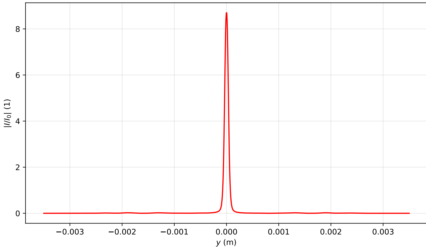
Intensity profile I(x=0, y, z=3.582)/I_0 , P_{in}=11.5P_{cr} , artificial time
