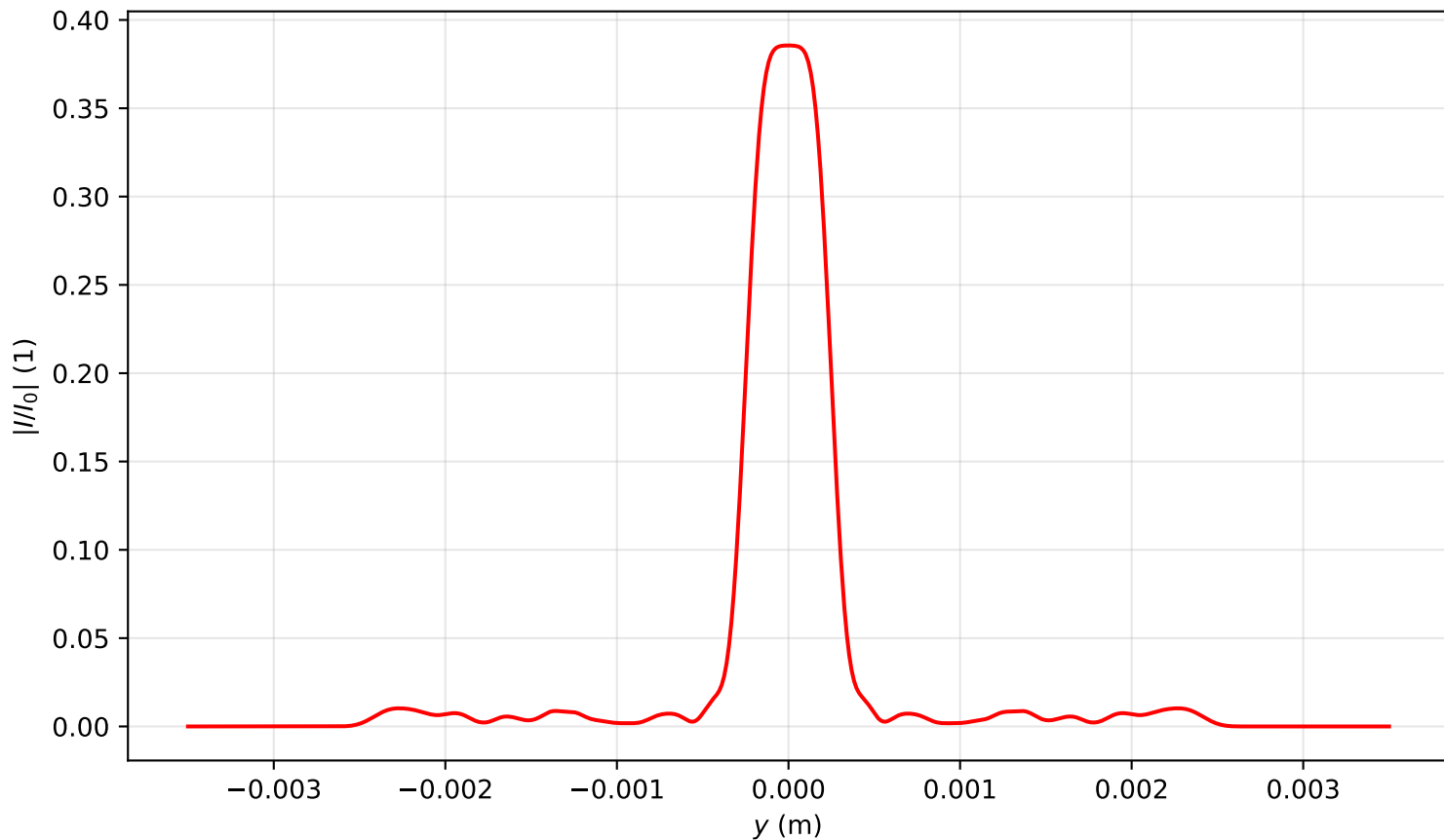
Intensity profile I(x=0, y, z=3.821)/I_0 , P_{in}=11.5P_{cr} , artificial time
