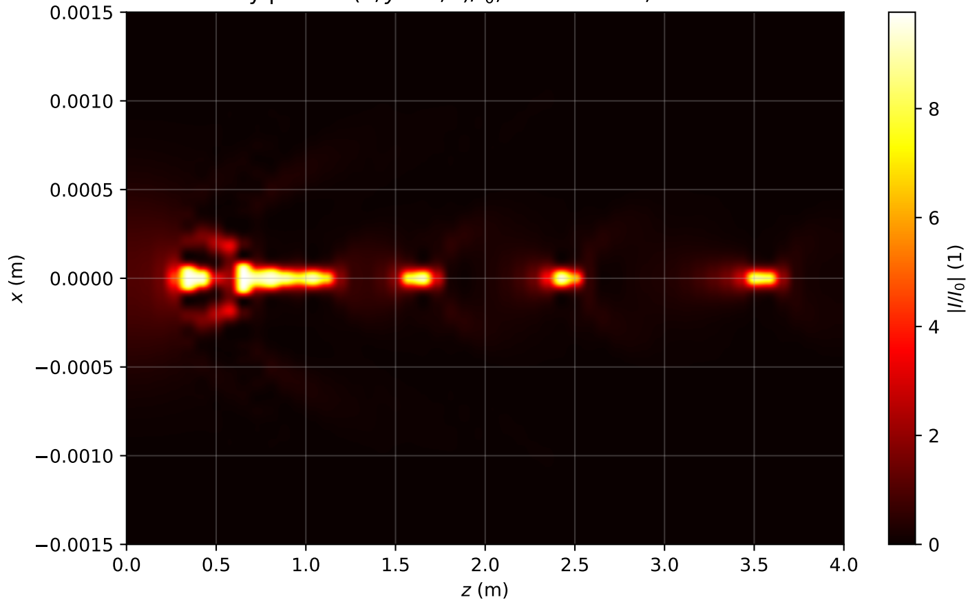
Intensity profile I(x, y = 0, z)/I_0 , P_{in}=11.5\text{Pcr} , artificial time
