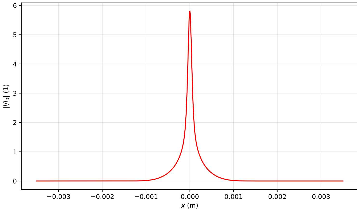
Intensity profile I(x, y = 0, z = 0.239)/I_0 , P_{in}=12.0P_{cr} , artificial time
