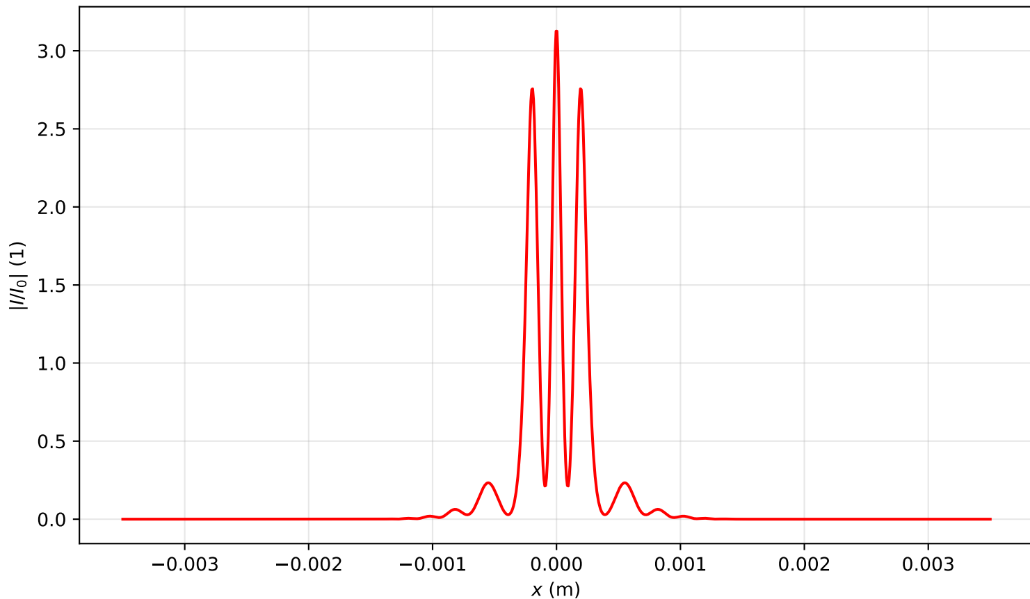
Intensity profile I(x, y = 0, z = 0.478)/I_0 , P_{in}=12.0P_{cr} , artificial time
