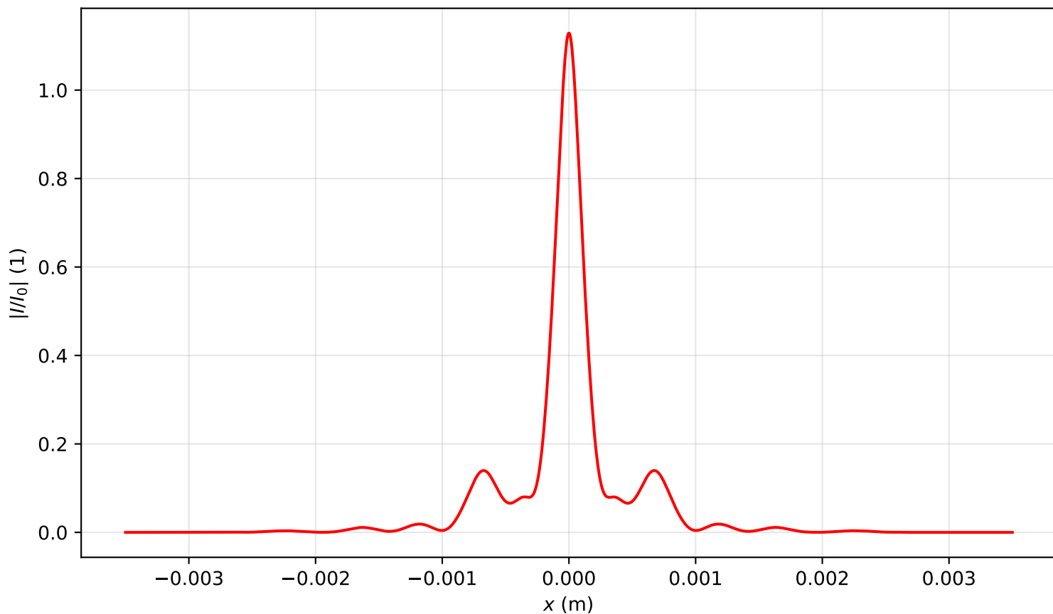
Intensity profile I(x, y = 0, z = 1.194)/I_0 , P_{in}=12.0P_{cr} , artificial time
