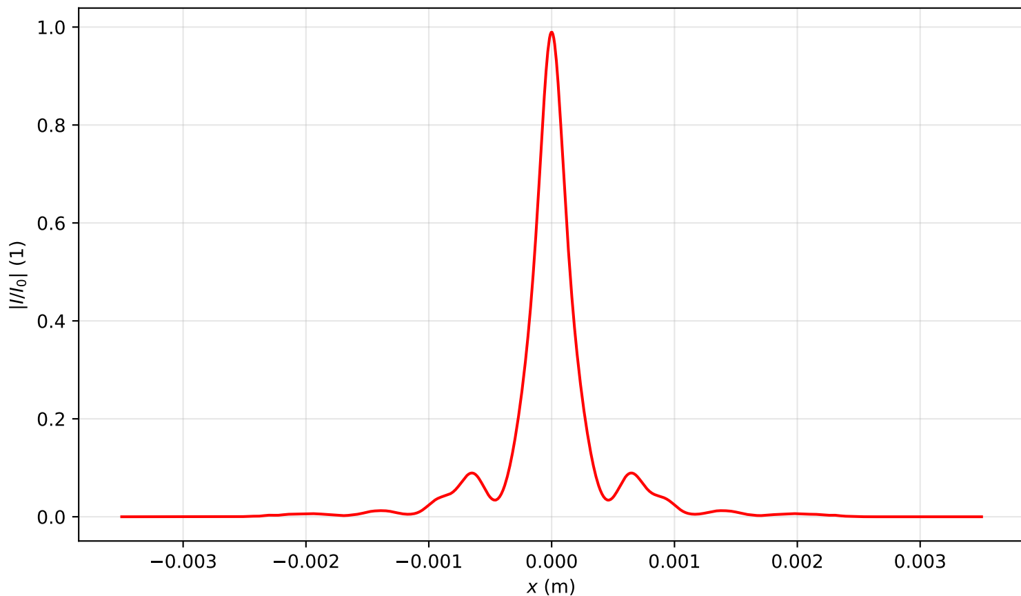
Intensity profile I(x, y = 0, z = 1.433)/I_0 , P_{in}=12.0P_{cr} , artificial time
