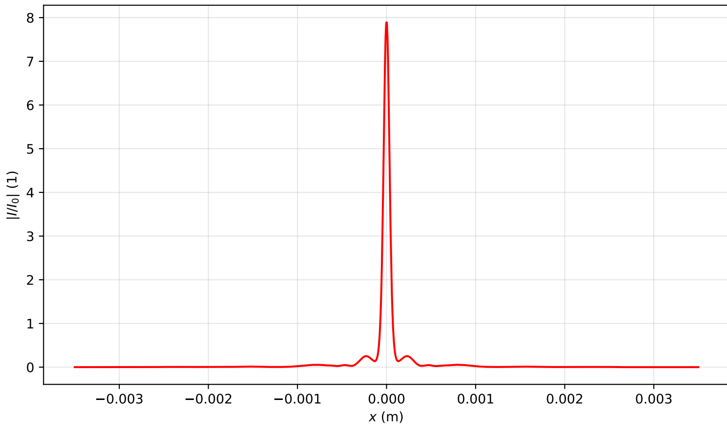
Intensity profile I(x, y = 0, z = 1.672)/I_0 , P_{in}=12.0P_{cr} , artificial time
