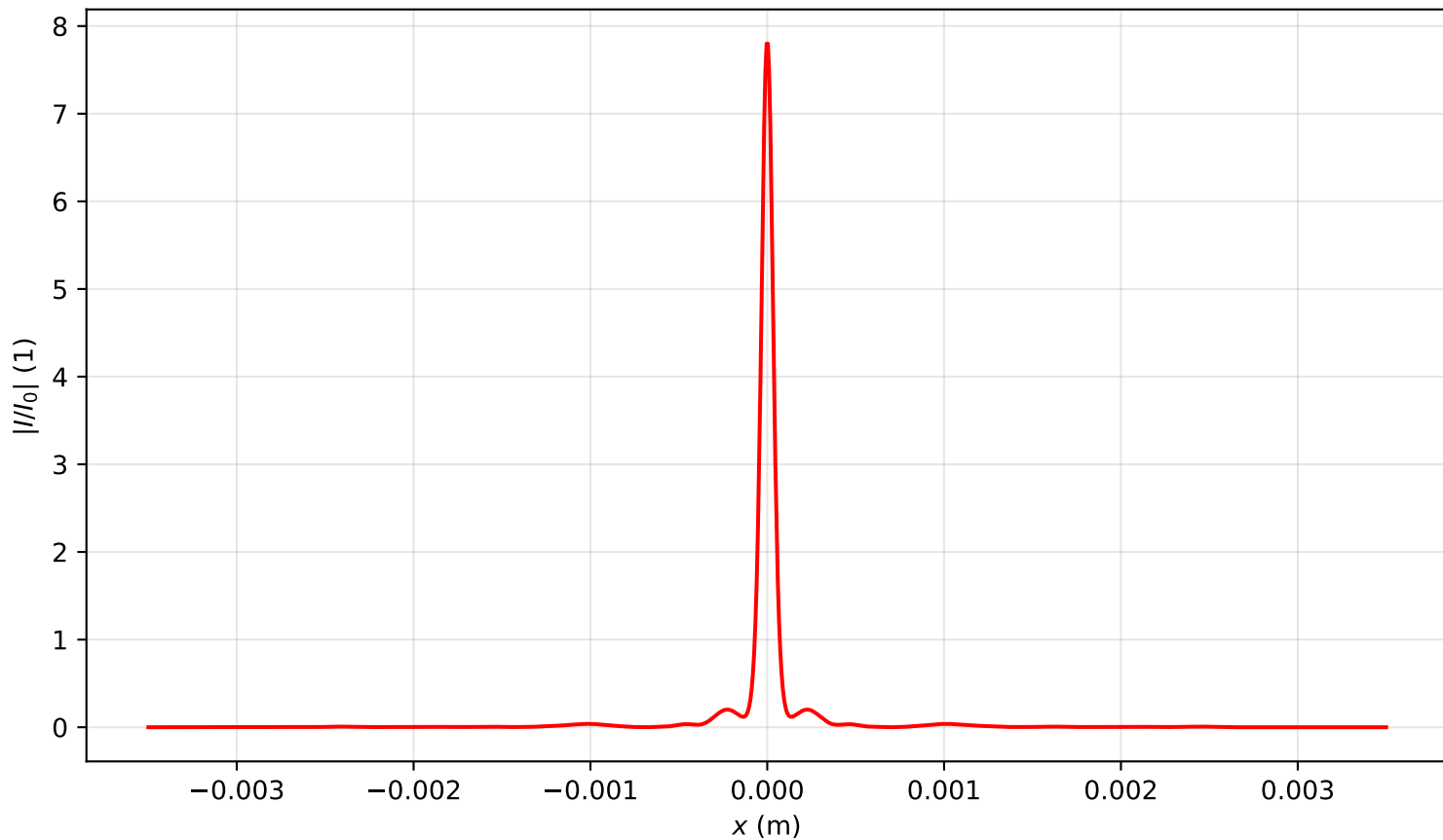
Intensity profile I(x, y = 0, z = 2.388)/I_0 , P_{in}=12.0P_{cr} , artificial time
