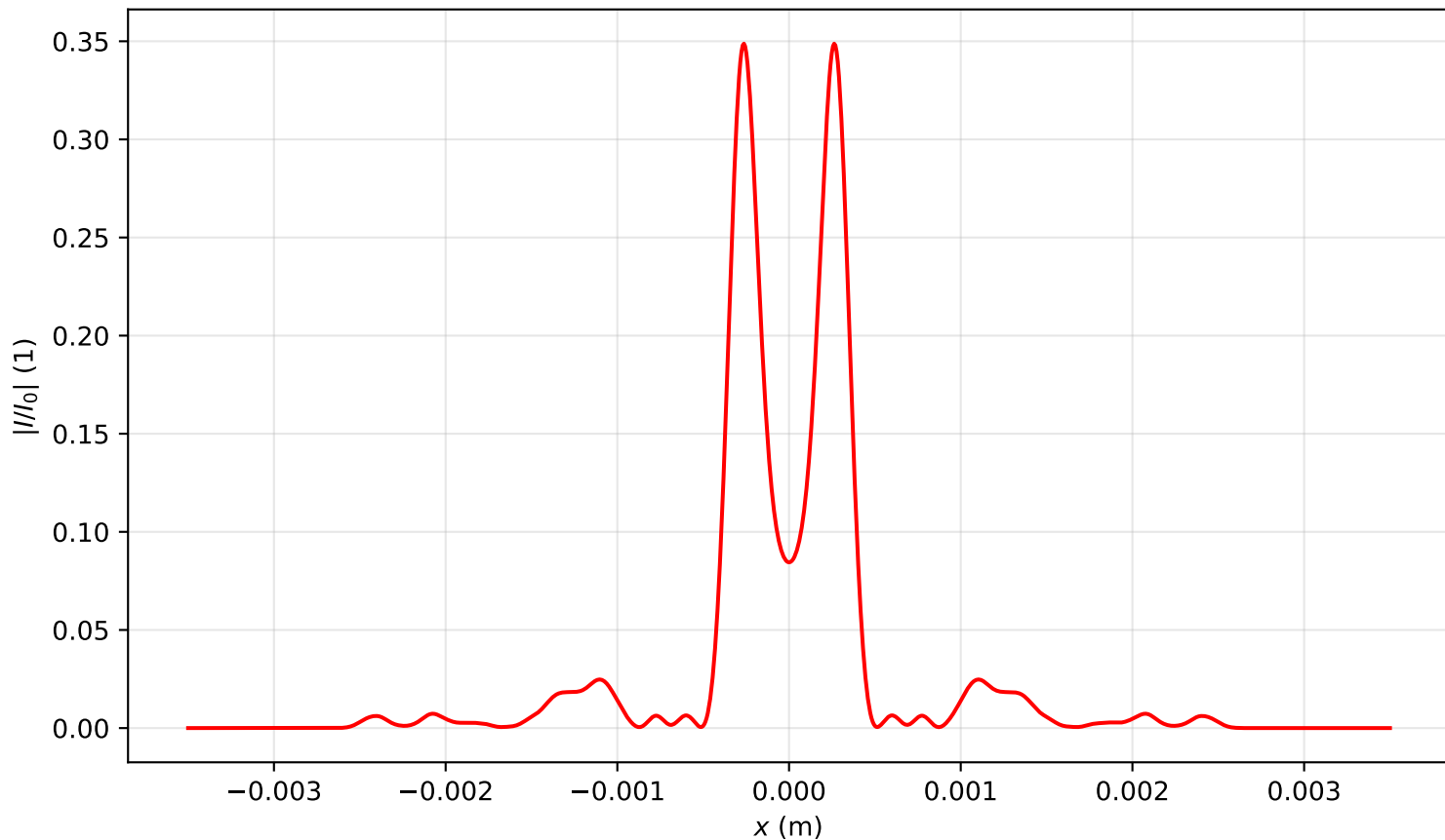
Intensity profile I(x, y = 0, z = 2.627)/I_0 , P_{in}=12.0P_{cr} , artificial time
