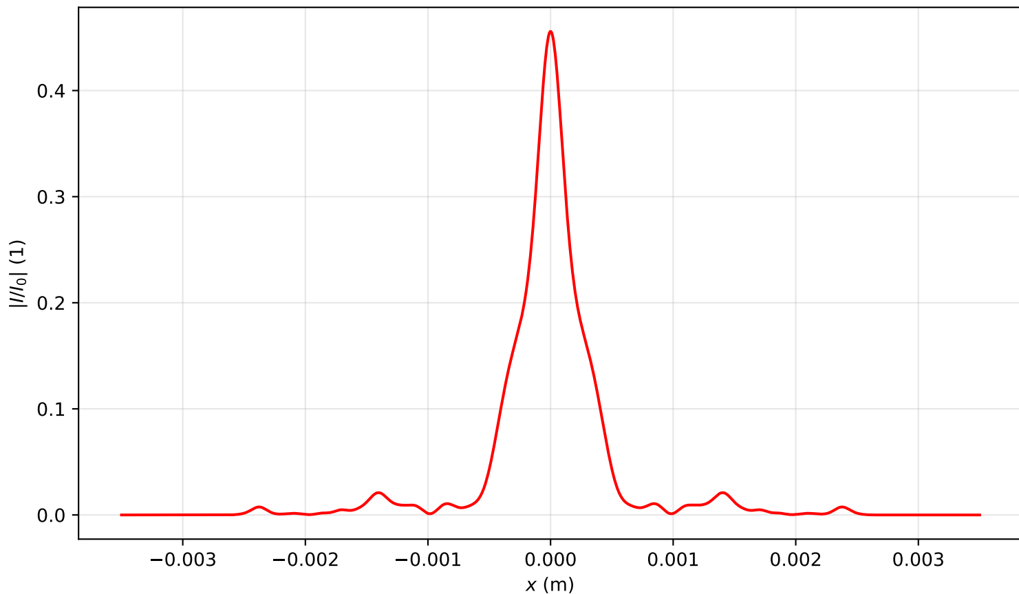
Intensity profile I(x, y = 0, z = 2.866)/I_0 , P_{in}=12.0P_{cr} , artificial time
