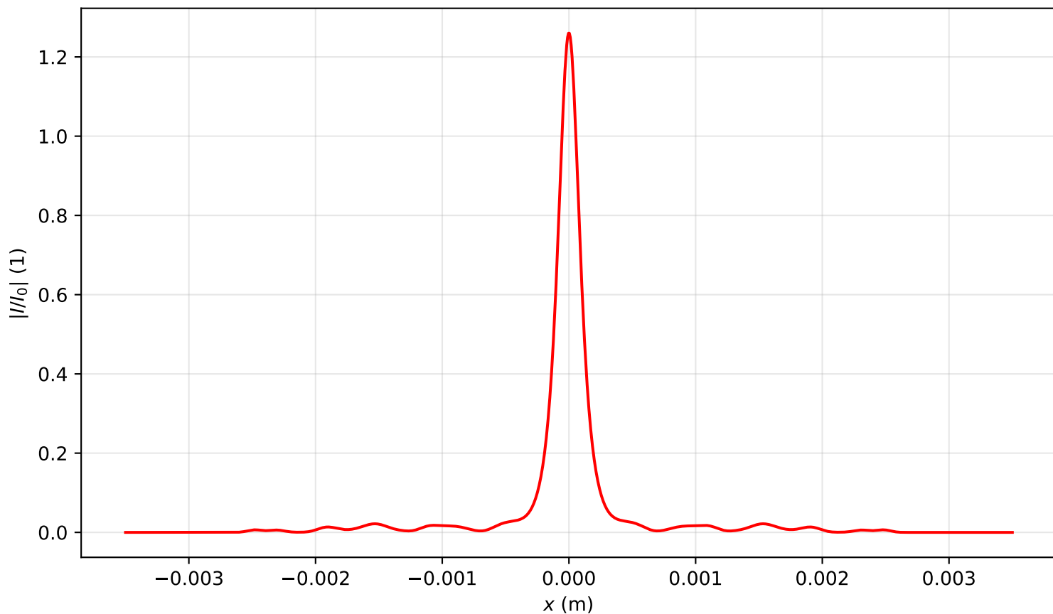
Intensity profile I(x, y = 0, z = 3.105)/I_0 , P_{in}=12.0P_{cr} , artificial time
