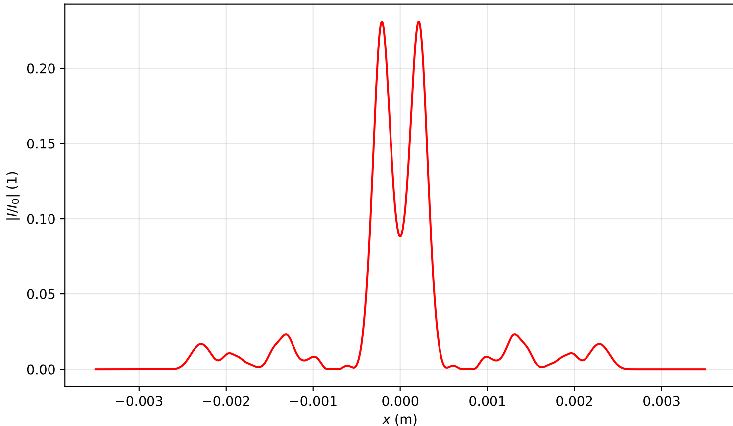
Intensity profile I(x, y = 0, z = 3.582)/I_0 , P_{in}=12.0P_{cr} , artificial time
