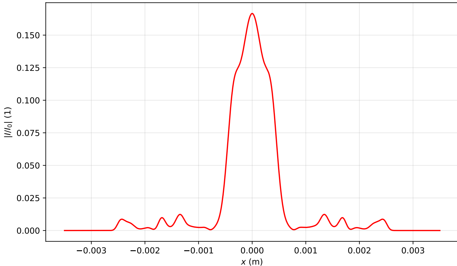
Intensity profile I(x, y = 0, z = 3.821)/I_0 , P_{in}=12.0\text{Pcr} , artificial time
