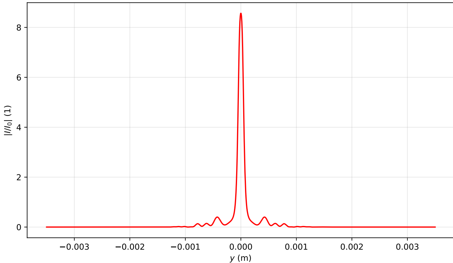
Intensity profile I(x=0, y, z=0.716)/I_0 , P_{in}=12.0P_{cr} , artificial time
