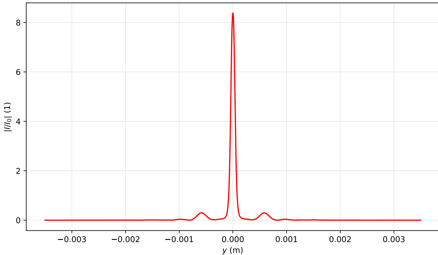
Intensity profile I(x=0, y, z=0.955)/I_0 , P_{in}=12.0P_{cr} , artificial time
